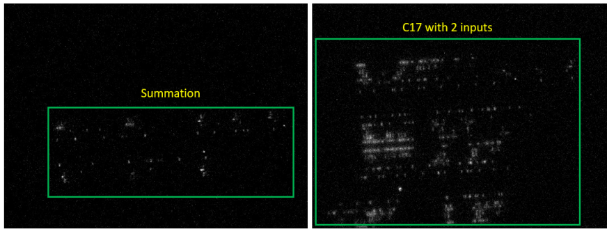
Figure 13: Raw images without cropping with the 20x zoom lens using the ALPhANOV microscope. The sub-figure on the left side shows the emission captured from the summation circuit, while the one on the right side shows the emission from the C17 circuit. The size and placement density of both circuits are visible clearly. The summation circuit is sparsely placed, while c17 is densely packed.
